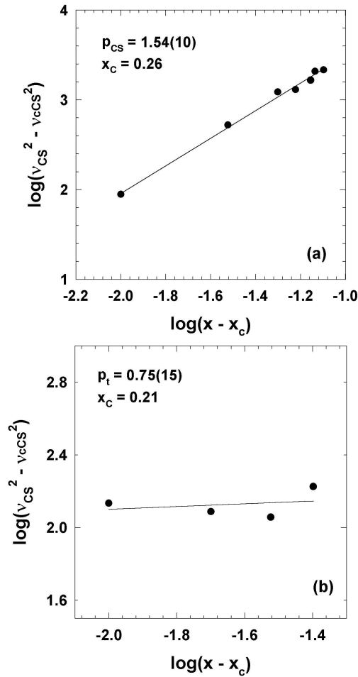
Fig. 7. Plots of \log_{10} (n^2 - n_{\text{C}}^2(x)) against \log_{10}(x - x_c) for the CS mode frequency in \text{Ge}_x\text{Se}_{1-x} glasses. The plots give respective power laws for CS - mode - based optical elasticity in the rigid region, p_{\text{CS}} , and in the transition region, p_t . Fig. taken from Ref. 41.
