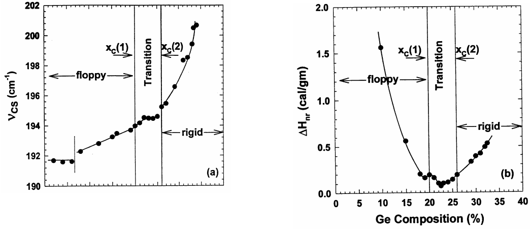
Fig. 6a). Raman mode frequency variation of corner-sharing ( n_{\text{CS}} ) tetrahedra in \text{Ge}_x\text{Se}_{1-x} plotted as a function of x ; b) Non-reversing heat variation, \Delta H_{\text{nr}}(x) , in \text{Ge}_x\text{Se}_{1-x} glasses. Fig. is taken from Ref. 41.
