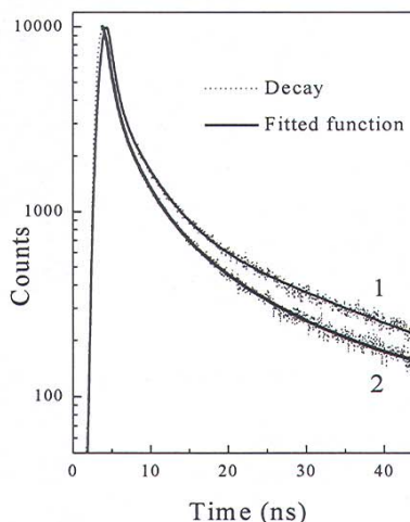
Fig. 4. Luminescence decays and fitted function CdSe NCs in a PMMA matrix at \lambda_{\text{exc}} = 375 nm (1) and 485 nm (2).
