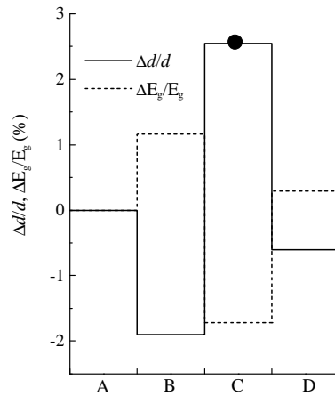
Fig. 1. Variation in relative changes in thickness d and optical bandgap E_g of a- \text{As}_2\text{Se}_3 (after [14]). Measurement conditions are described in the text.
