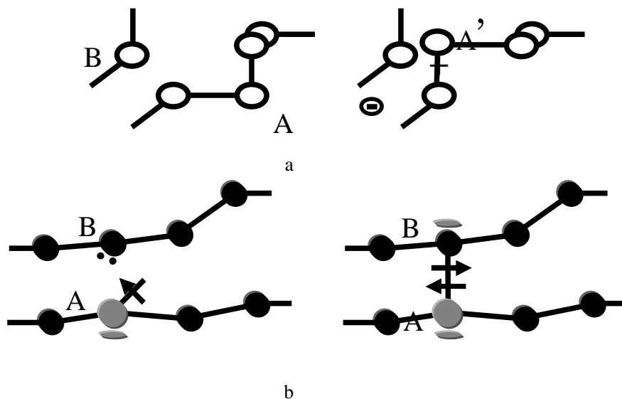
Fig. 8. (a) Bond-twisting model (after [2]) and (b) bond-breaking model (after [10]) which are applied to a-Se.
