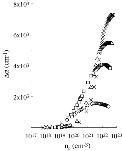
Fig. 4. In situ variation of changes in absorption coefficient \Delta\alpha as a function of absorbed photons n_p at various temperatures. \times , \Delta , \square , and O show the changes at 50, 100, 200, and 300 K, respectively. Illumination is by \text{Ar}^+ laser ( 20\text{mW}/\text{cm}^2 ) (after [13]).
