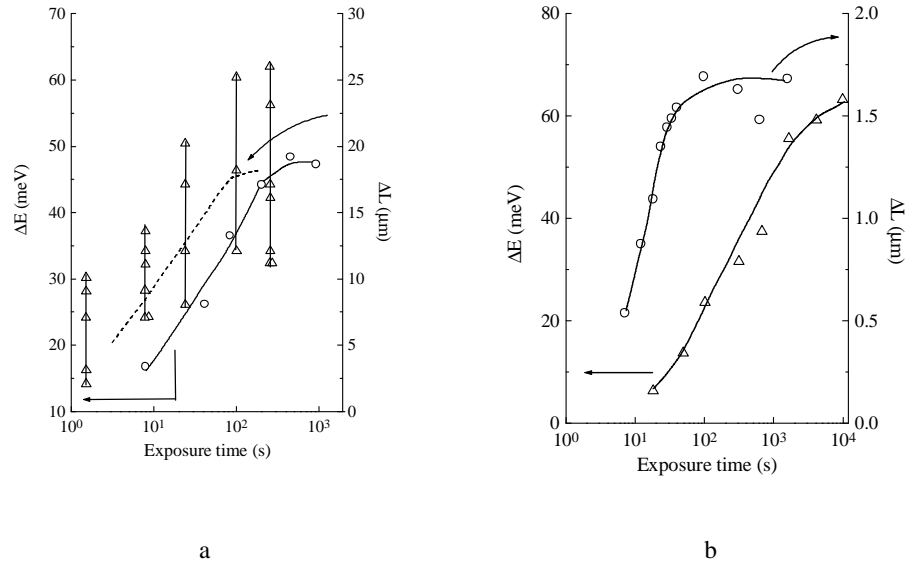
Fig. 2. Photoexpansion \Delta L and photodarkening \Delta E as a function of exposure time in a-As 2 S 3 for (a) bandgap and (b) subgap illumination (after [8]).
