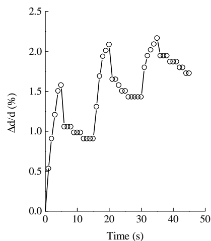
Fig. 7. Relative changes in thickness \Delta d/d with time for short duration of illumination for a-As 2 S 3 . Light ON and OFF states is 5 and 10 s, respectively (after [12]).
