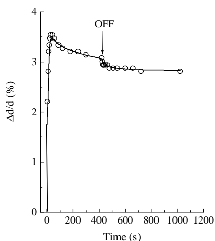
Fig. 6. Relative changes in thickness \Delta d/d with time for a-As 2 S 3 (after [12]).
