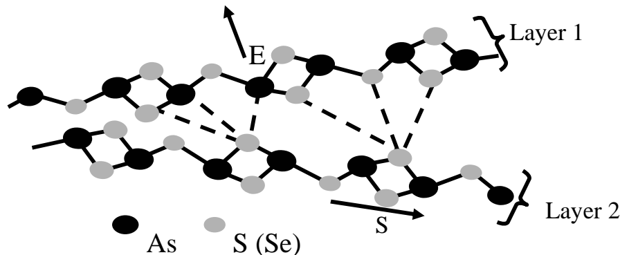
Fig. 9. The repulsion and slip motion of layered cluster model (after [11]). The arrows E and S indicate the expansion (due to repulsion) and the slip motions, respectively. The difference in local environments (and hence LP interactions) between chalcogen atoms is indicated by the broken lines.
