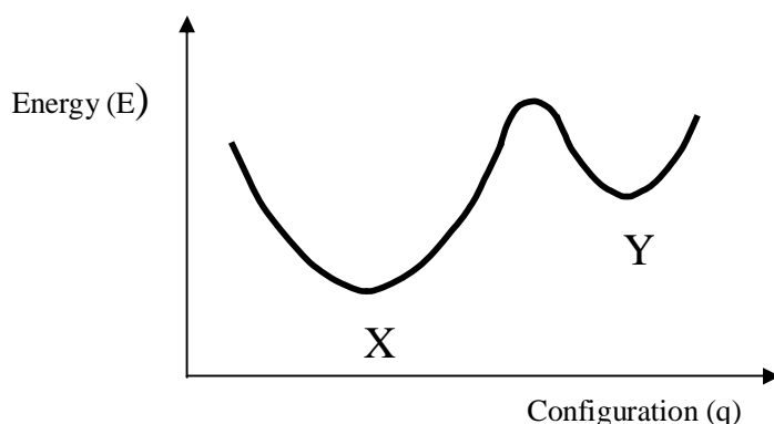
Fig. 10. Configurational-coordinate potential-energy diagram illustrating schematically the relative energies of the ground-state (X) and the photo-excited state (Y).
