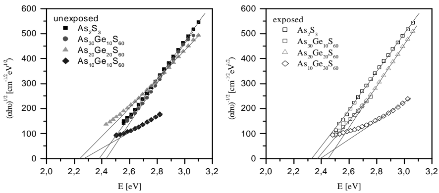
Fig. 3. Optical absorption edge (\alpha h\nu)^{1/2} vs. energy of photon ( h\nu ) for unexposed and exposed thin As-Ge-S films
