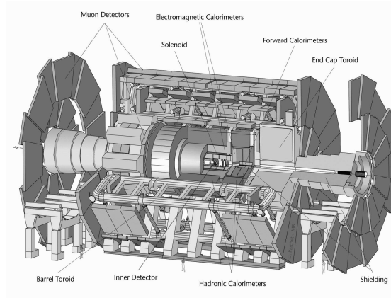
Fig. 2. The ATLAS detector for LHC, CERN, Characteristics: width 44 m, diameter 22 m, weight 7000t [14].
