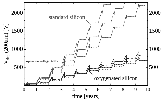
Fig. 13. Damage projections for the ATLAS pixel detector ( r = 4 \text{ cm} ), yearly warm up: 14, 30 and 60 days [22].
