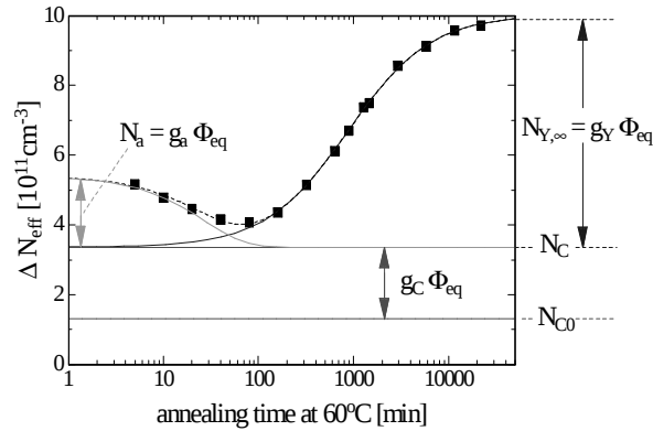
Fig. 10. Change of the measured space charge concentration as function of annealing time at T = 60^\circ\text{C} [28].
