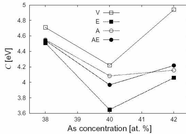
Fig. 6. The dependences of parameter C on the As concentration.
