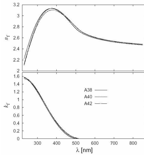
Fig. 2. The spectral dependences of the refractive index n_f and extinction coefficient k_f calculated on the basis of the material parameters found for the annealed samples.
