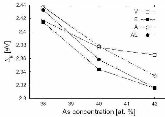
Fig. 3. The dependences of the band gap E_g on the As concentration.
