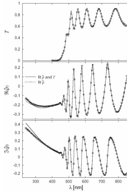
Fig. 1. The spectral dependences of the transmittance T and real part \Re and imaginary part \Im of the ellipsometric ratio \hat{p} for sample V38: points denote experimental values and lines represent the calculated values using the parameter values found by LSM.
