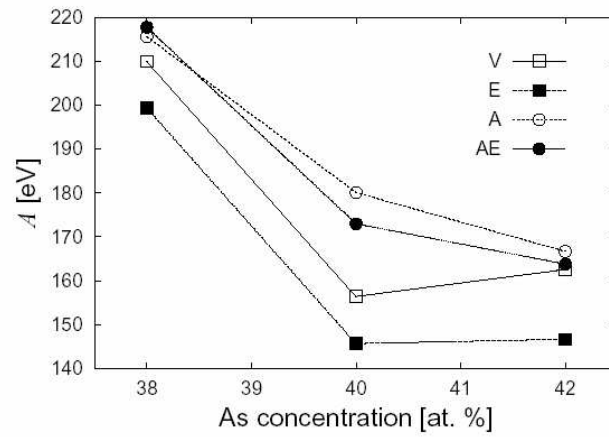
Fig. 5. The dependences of parameter A on the As concentration.
