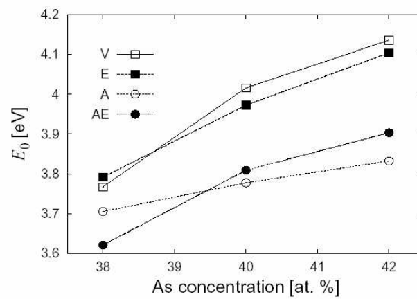
Fig. 4. The dependences of parameter E_0 on the As concentration.
