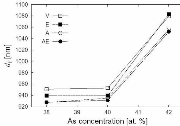
Fig. 9. The dependences of the thickness d_f on the As concentration.
