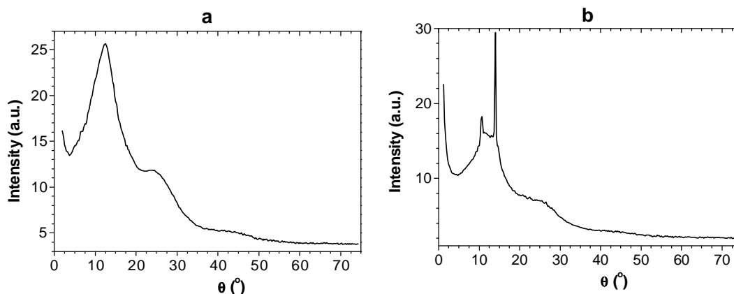
Fig. 1. a. the X-ray diffraction pattern of the as-prepared thin film \text{Se}_{42}\text{S}_{58} doped by paraffins. b. the X-ray diffraction pattern of the annealed film \text{Se}_{42}\text{S}_{58} doped by paraffins.
