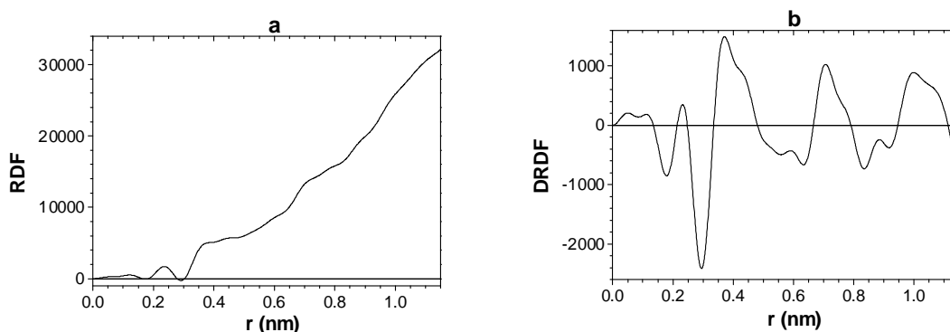
Fig. 3. Radial distribution function (RDF) (a) and difference radial distribution function (DRDF) (b) in annealed PLD deposited thin films of hybrid chalcogenide-paraffin amorphous material.
