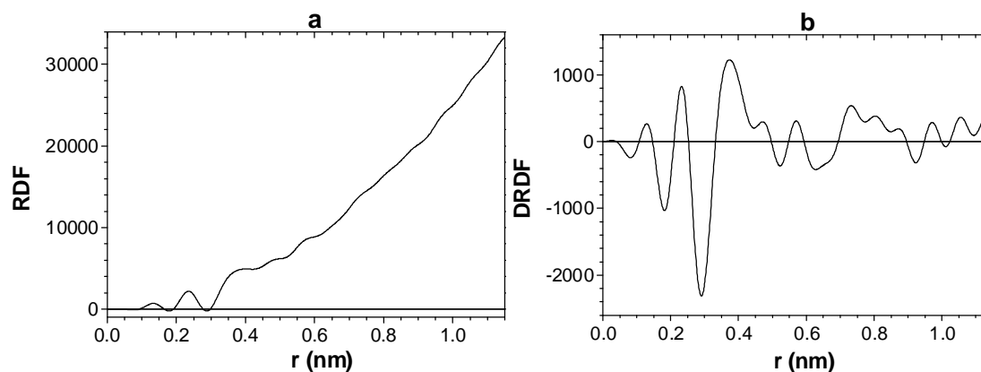
Fig. 2. Radial distribution function (RDF) (a) and difference radial distribution function (DRDF) (b) in fresh PLD deposited thin films of hybrid chalcogenide-paraffin amorphous material.
