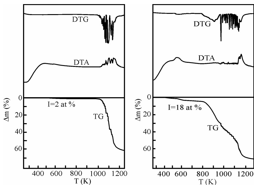
Fig. 8. DTG, TG and DTA curves for Ge_{20}As_{14}(S_{0.5}Se_{0.5})_{66-x}I_x .
