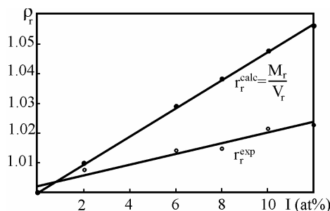
Fig. 4. Experimental ( \rho_r^{\text{exp}} ) and calculated ( \rho_r^{\text{calc}} ) relative densities of the glasses in the \text{Ge}_{20}\text{As}_{14}(\text{S}_{0.5}\text{Se}_{0.5})_{66-x}\text{I}_x system as a function of iodine content.
