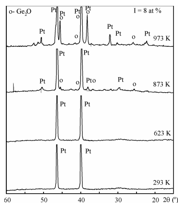
Fig. 11. High-temperature diffractogram of the glass \text{Ge}_{20}\text{As}_{14}\text{S}_{29}\text{Se}_{29}\text{I}_8 .
