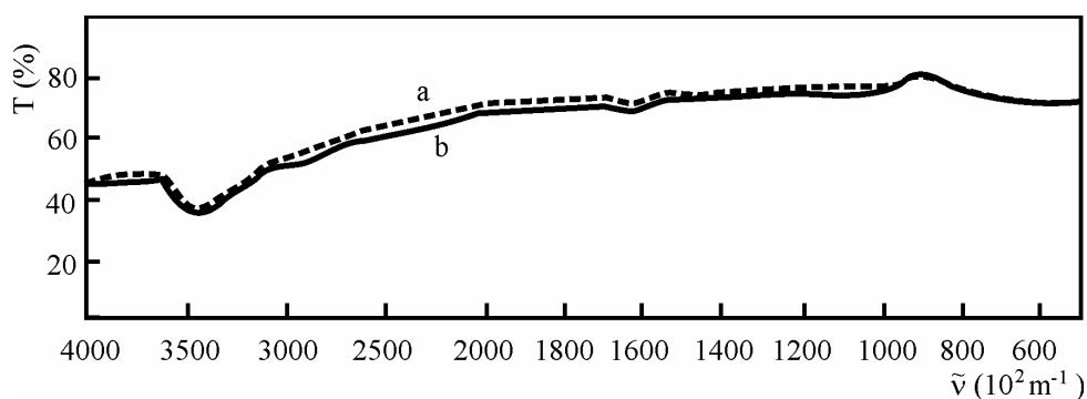
Fig. 14. IR spectrum of \text{Ge}_{20}\text{As}_{14}(\text{S}_{0.5}\text{Se}_{0.5})_{66-x}\text{I}_x , for x=6 (a) and x=12 (b).
