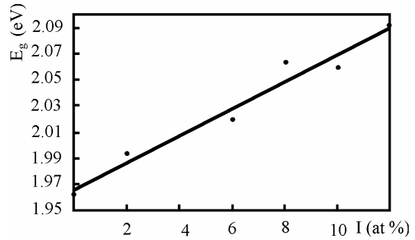
Fig. 16. Optical bandgap as a function of iodine concentration for the glasses of the system \text{Ge}_{20}\text{As}_{14}(\text{S}_{0.5}\text{Se}_{0.5})_{66-x}\text{I}_x .
