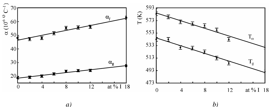
Fig. 13. Dependence of thermal coefficient of linear expansion (a) and of T_g and T_\infty (b) of the glass \text{Ge}_{20}\text{As}_{14}(\text{S}_{0.5}\text{Se}_{0.5})_{66-x}\text{I}_x on iodine content.
