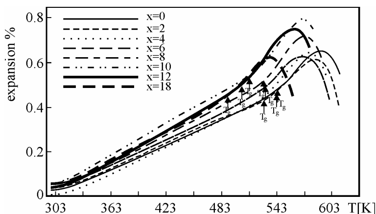
Fig. 12. DTD curves of the glasses \text{Ge}_{20}\text{As}_{14}(\text{S}_{0.5}\text{Se}_{0.5})_{66-x}\text{I}_x .
