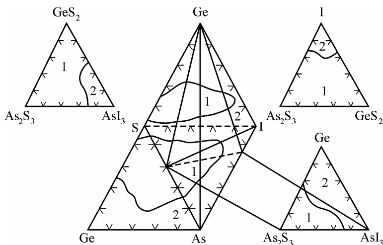
Fig. 1. The glass-forming region in the system Ge-As-S-I: 1 – glass; 2 – crystal.
