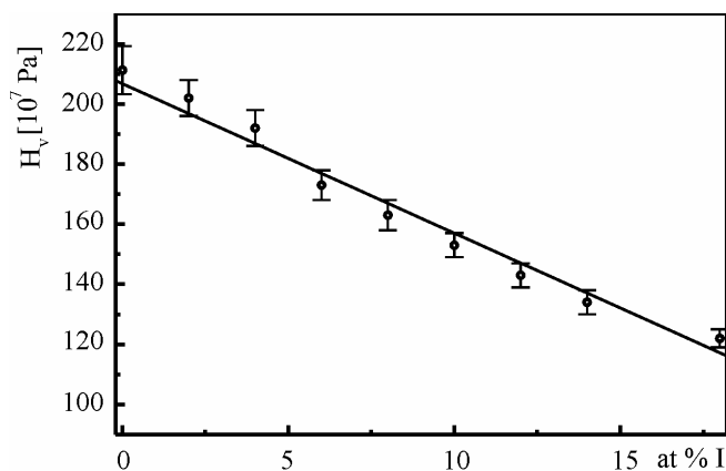
Fig. 6. Dependence of microhardness of the glasses from the system \text{Ge}_{20}\text{As}_{14}(\text{S}_{0.5}\text{Se}_{0.5})_{66-x}\text{I}_x on iodine content.
