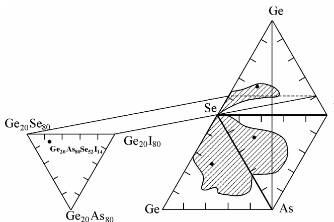
Fig. 2. The glass-forming region in the system Ge-As-Se-I.
