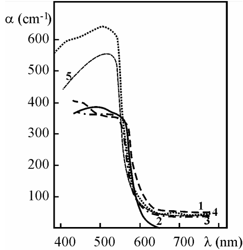
Fig. 15. Dependence of the absorption coefficient on wavelength for the glasses of the system \text{Ge}_{20}\text{As}_{14}(\text{S}_{0.5}\text{Se}_{0.5})_{66-x}\text{I}_x , for: 1) x = 0 ; 2) x = 2 ; 3) x = 6 ; 4) x = 10 ; 5) x = 14 .
