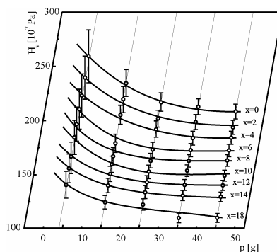
Fig. 5. Dependence of microhardness of the glasses from the system \text{Ge}_{20}\text{As}_{14}(\text{S}_{0.5}\text{Se}_{0.5})_{66-x}\text{I}_x on the indenter mass load.
