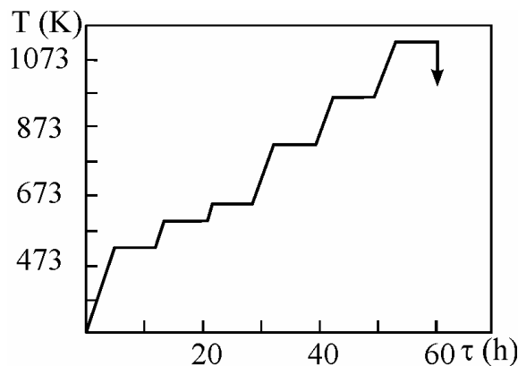
Fig. 3. Diagram of process for obtaining glasses of \text{Ge}_{20}\text{As}_{14}(\text{S}_{0.5}\text{Se}_{0.5})_{66-x}\text{I}_x type.
