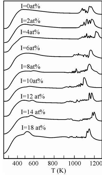
Fig. 9. DTA curves for the glasses of the type \text{Ge}_{20}\text{As}_{14}(\text{S}_{0.5}\text{Se}_{0.5})_{66-x}\text{I}_x .
