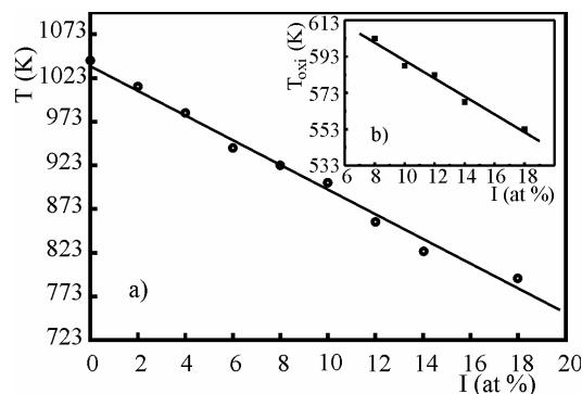
Fig. 10. Temperatures of the beginning of decomposition (a) and iodine oxidation in the glass \text{Ge}_{20}\text{As}_{14}(\text{S}_{0.5}\text{Se}_{0.5})_{66-x}\text{I}_x (b).
