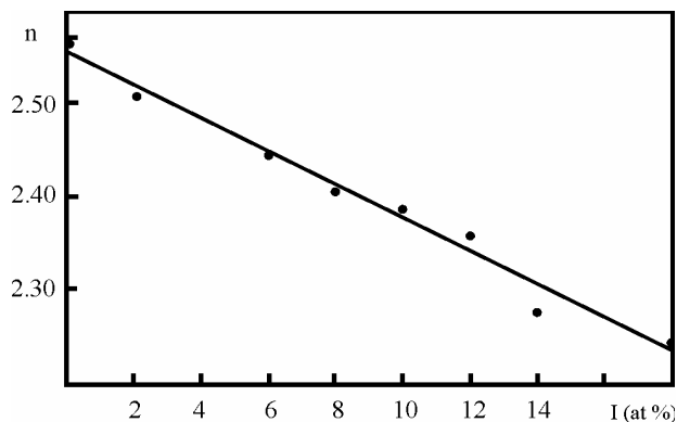
Fig. 17. Dependence of the refractive index on percentage of iodine in the sample.
