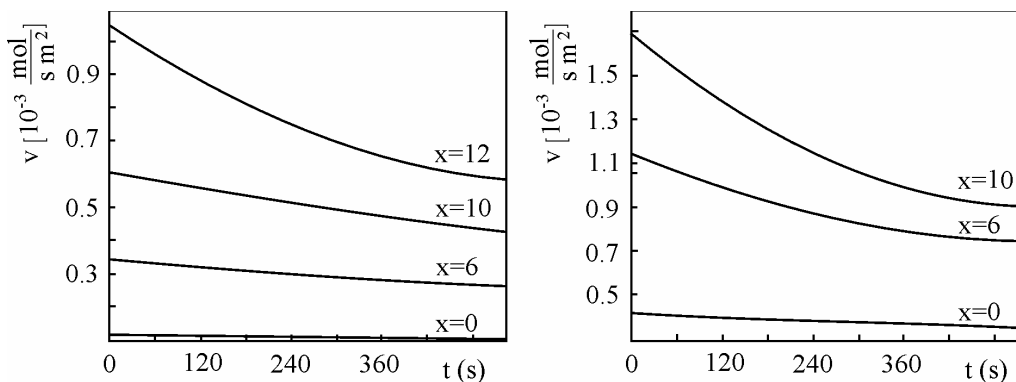
Fig. 7. Rate of dissolution of glasses of the system \text{Ge}_{20}\text{As}_{14}(\text{S}_{0.5}\text{Se}_{0.5})_{66-x}\text{I}_x as a function of time a) in 2 [mol/dm 3 ] KOH; b) in 5 [mol/dm 3 ] KOH.
