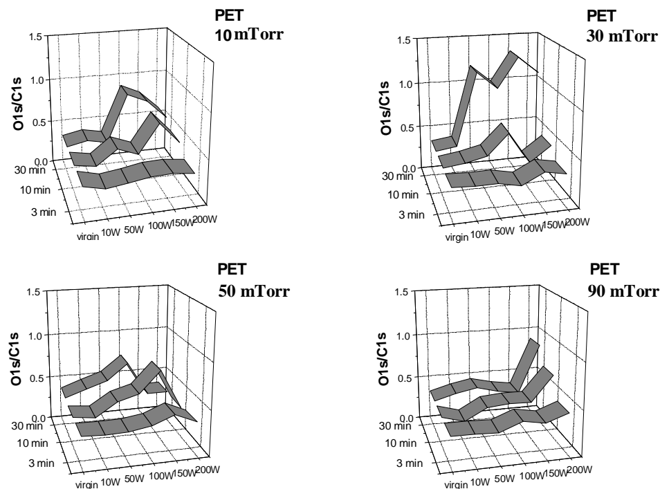
Fig. 2. The O1s/C1s ratios after different plasma treatment conditions and different treatment times.
