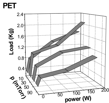
Fig. 9. Load test results for PET.
