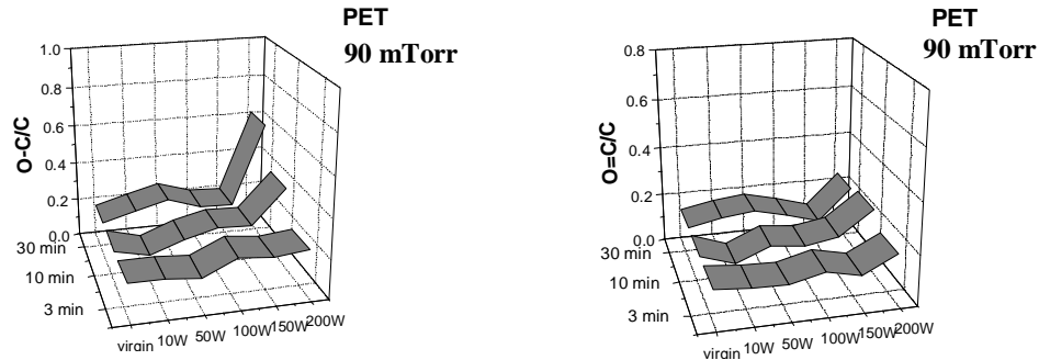
Fig. 6. The O-C/C and O=C/C ratios after plasma treatment at 90 mTorr
