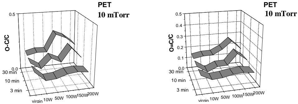
Fig. 3. The O-C/C and O=C/C ratios after plasma treatment at 10 mtorr.
