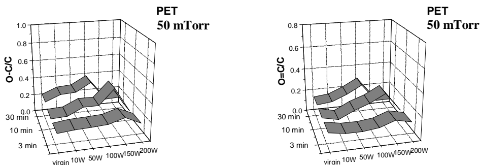
Fig. 5. The O-C/C and O=C/C ratios after plasma treatment at 50 mtorr.
