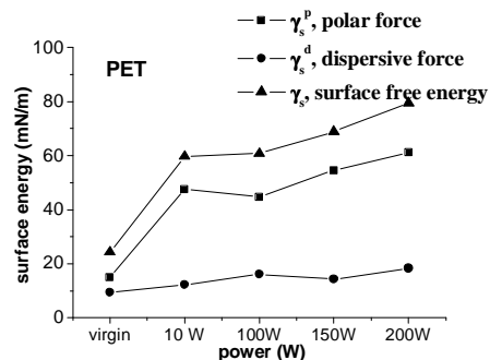
Fig. 7. Surface energy variation versus rf power.
