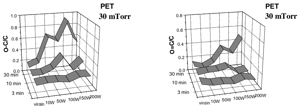
Fig. 4. The O-C/C and O=C/C ratios after plasma treatment at 30 mtorr.
