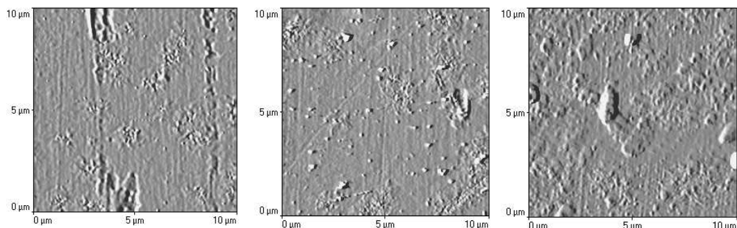
Fig. 8. AFM Images for PET surface before and after the plasma treatment: a) untreated; b) 30 mTorr, 100 W; c) 30 mTorr, 150 W.
